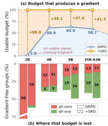
Figure 4: Uniform-reward groups waste most of the rollout at both ends of the capability range: (a) usable share of the budget, (b) overall training group composition.
