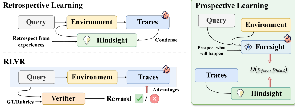
Figure 1: Comparison of three paradigms for converting agent experience into training signals. Reinforcement Learning with Verifiable Rewards (RLVR) scalarizes completed trajectories into outcome rewards and assigns them back to the action policy. Retrospective Learning retains structured post-hoc hindsight to supervise behavior. Prospective Learning uses hindsight to supervise predictions formed from information available before interaction.
