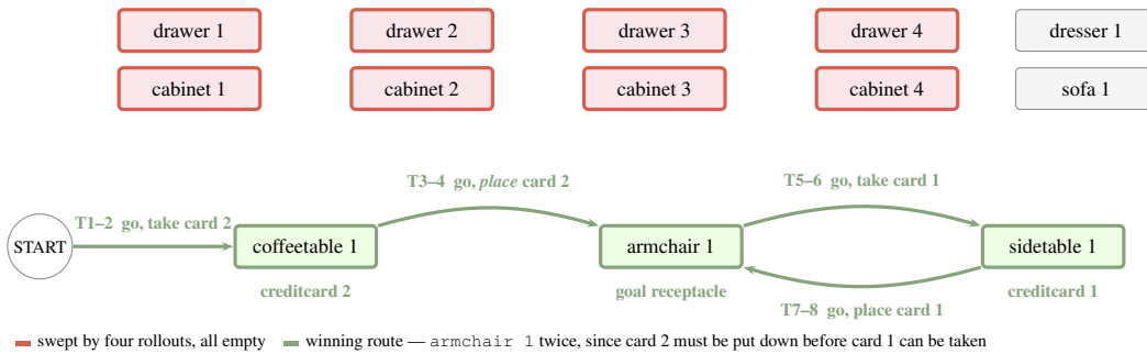
Figure 5: Both cards sit on furniture named in the opening observation. Four of the eight rollouts nonetheless sweep drawer 1--4 or cabinet 1--4 and never reach them. The winning route returns to armchair 1 a second time: the first card has to be deposited before the second can be picked up, so the detour is forced, and the four legs consume the eight-action budget exactly.
