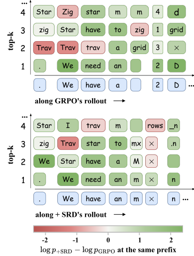
Figure 3: The same shift token by token, on one rollout per arm: rows are the top-4 likeliest continuations under the policy that owns the rollout.
