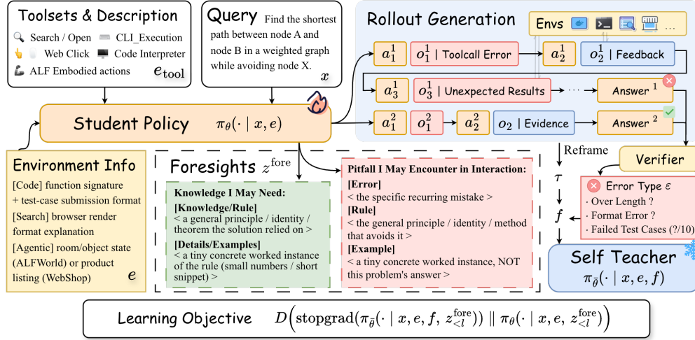
Figure 2: Overview of Self-Retrospection Distillation (SRD). The student policy rolls out trajectories and generates anticipated pitfalls and knowledge foresights via a differently prompted call to the same model. Post-hoc experience from the completed trajectory conditions the stopped-gradient self-teacher, whose token-level distributions supervise the student’s own foresight rollout.
