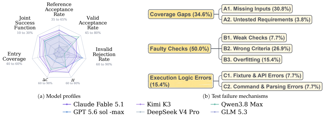
Figure 4. Model profiles across all 300 benchmark tasks (a) and failure mechanisms in 286 sampled failed trajectories after excluding 14 timeouts (b).
