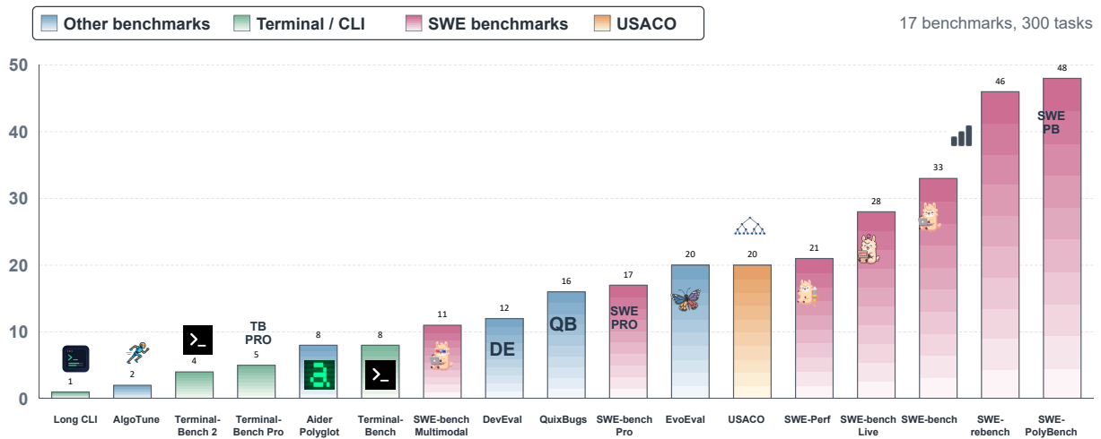
Figure 6. Test tasks by source benchmark.
