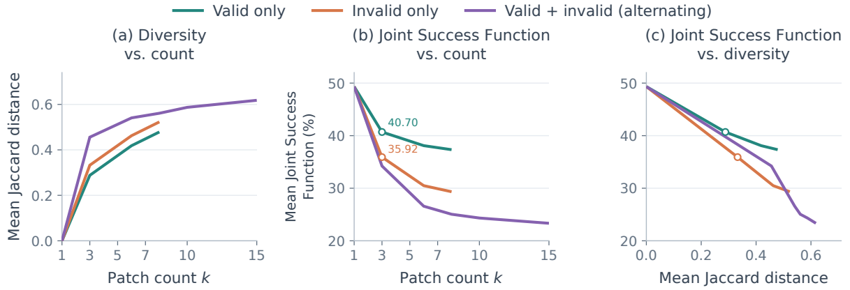
Figure 3. Joint Success Function and candidate diversity under three patch addition schedules.
