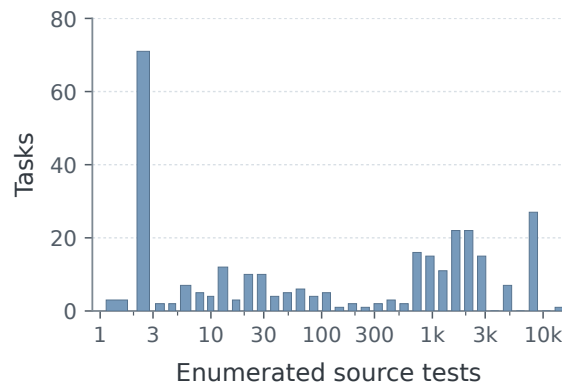
Figure 5. Distribution of source test counts.
