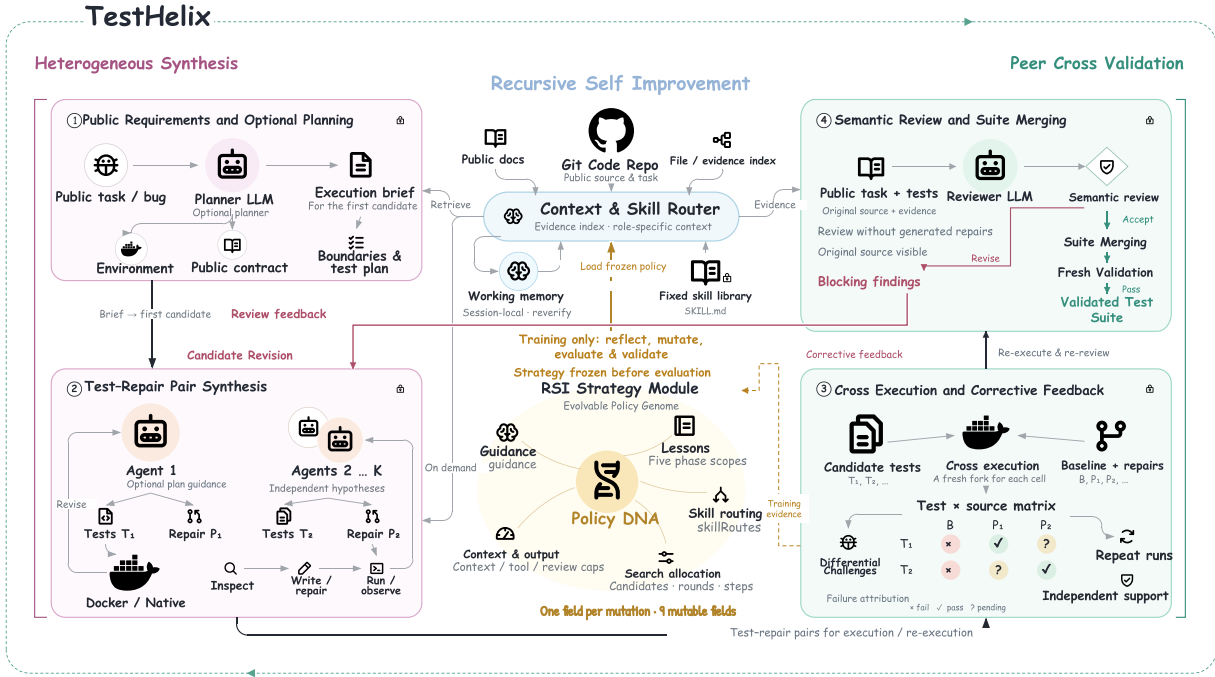
Figure 2. TestHelix architecture.
