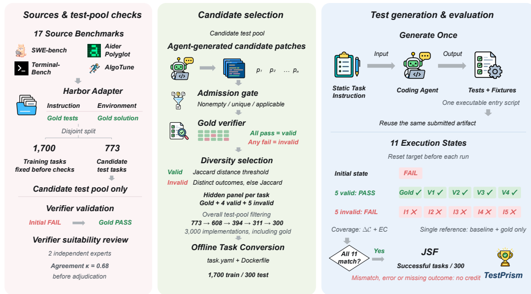
Figure 1. Overview of TestPrism construction and evaluation.
