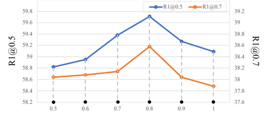
Fig. 6 Results of different values of the hyperparamete \tau .
