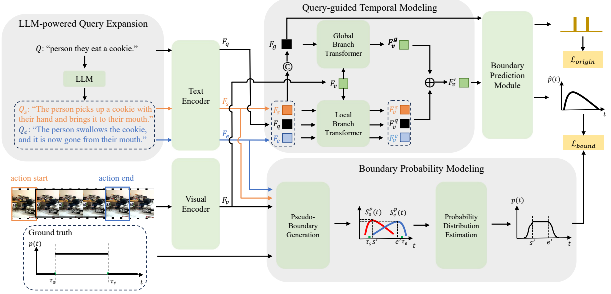
Fig. 2 Overview of the proposed action localization framework. The pipeline first leverages a large language model to perform text expansion, generating detailed sentences that describe the beginning and ending stages of the target action based on the original content-focused query. These expanded boundary cues, along with the visual video, are processed by the base model to obtain initial text and video features. To refine the multimodal representations, we introduce a query-guided temporal modeling module that fuses the detailed start and end descriptions with the video features, employing global and local branches to capture holistic context and stage-specific boundary details. Finally, a boundary probability modeling module is proposed to estimate the likelihood of action boundaries across the temporal sequence, converting rigid ground-truth intervals into soft probability scores for more robust supervision during training.
