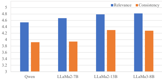
(a) GPT-4-based Evaluation Results
