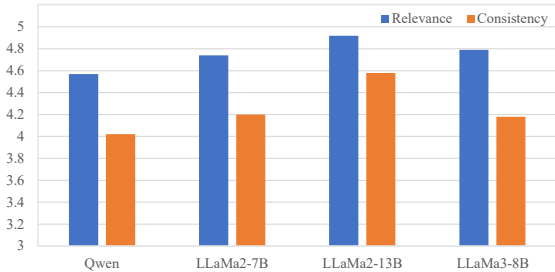
(b) Human Evaluation Results
