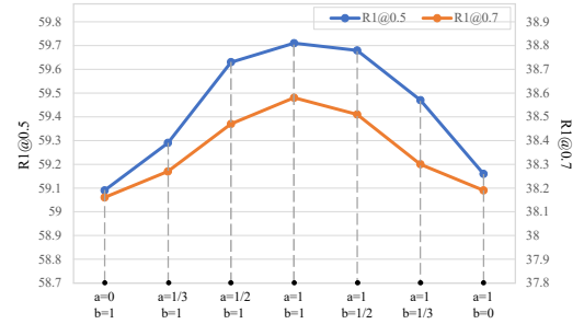
Fig. 4 Results of different values of hyperparameters ( a and b ) for the global and local branches with QD-DETR on the Charades-STA dataset.
