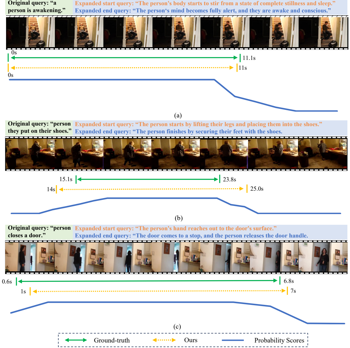
Fig. 10 Visualization of boundary probability scores on the Charades-STA dataset by integrating our modules into QD-DETR.
