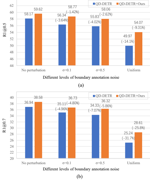
Fig. 7 Results of boundary annotation perturbation on the Charades-STA dataset by integrating our modules into QD-DETR.
