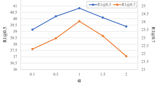
Fig. 5 Results of different values of the hyperparameter ( \alpha ) for the global and local branches with QD-DETR on the Charades-STA dataset.
