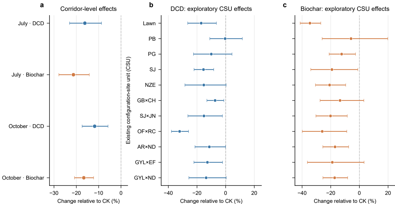
a, CSU-clustered 95% confidence intervals (11 CSUs). b–c, descriptive t intervals from three block-level summaries per CSU; no CSU-wise significance tests.
