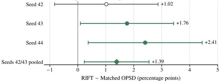
(a) Positive gain in all training seeds
