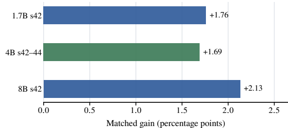
(b) Gain transfers across model scale
