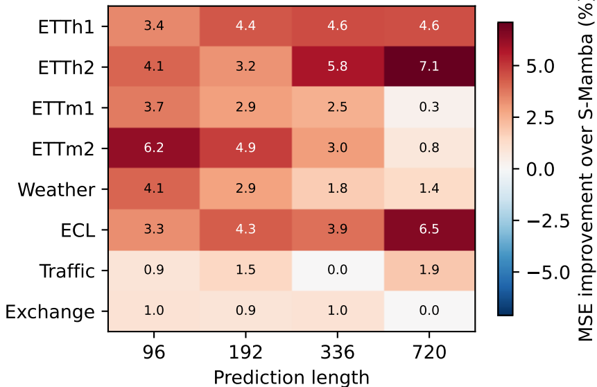
QCK-M vs S-Mamba
