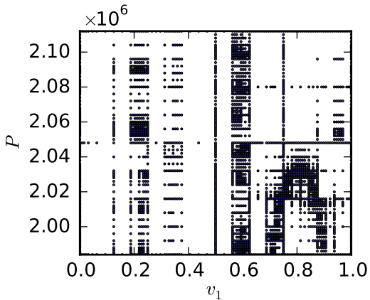
xW1 sparse grid
