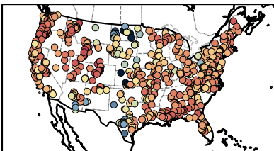
(e) mKGE
