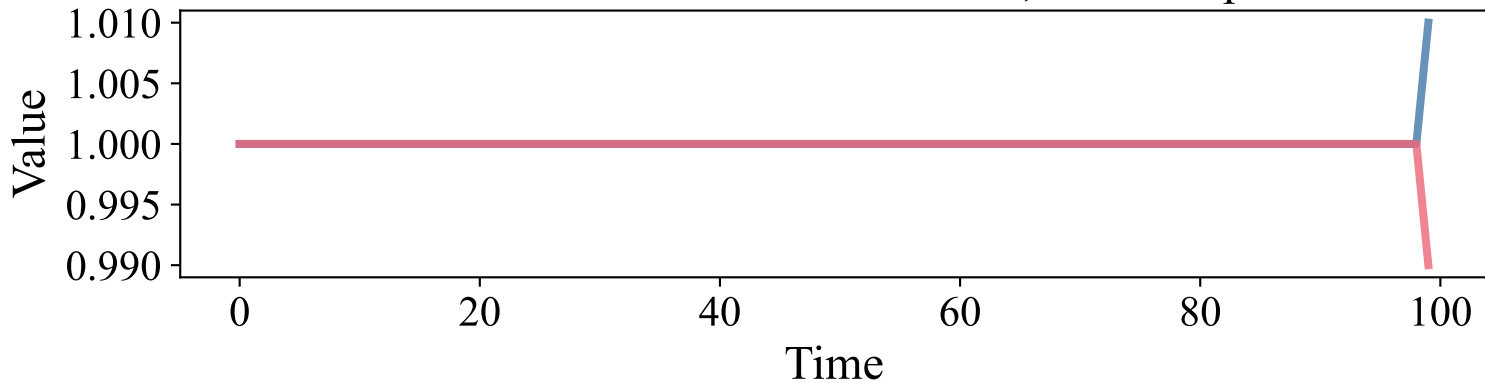
(a) Runoff data with a small outlier, different phase.
