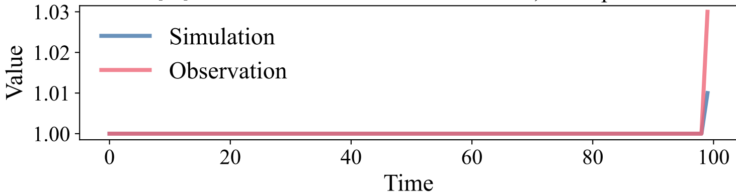
(b) Runoff data with an extreme event, same phase.
