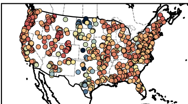
(e) mKGE
