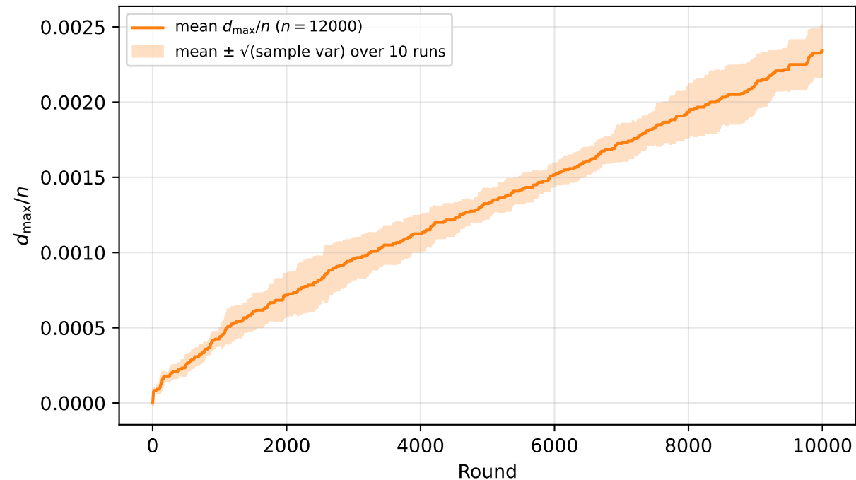
d_{\max}/n vs round (MovieLens, n = 12000 )
