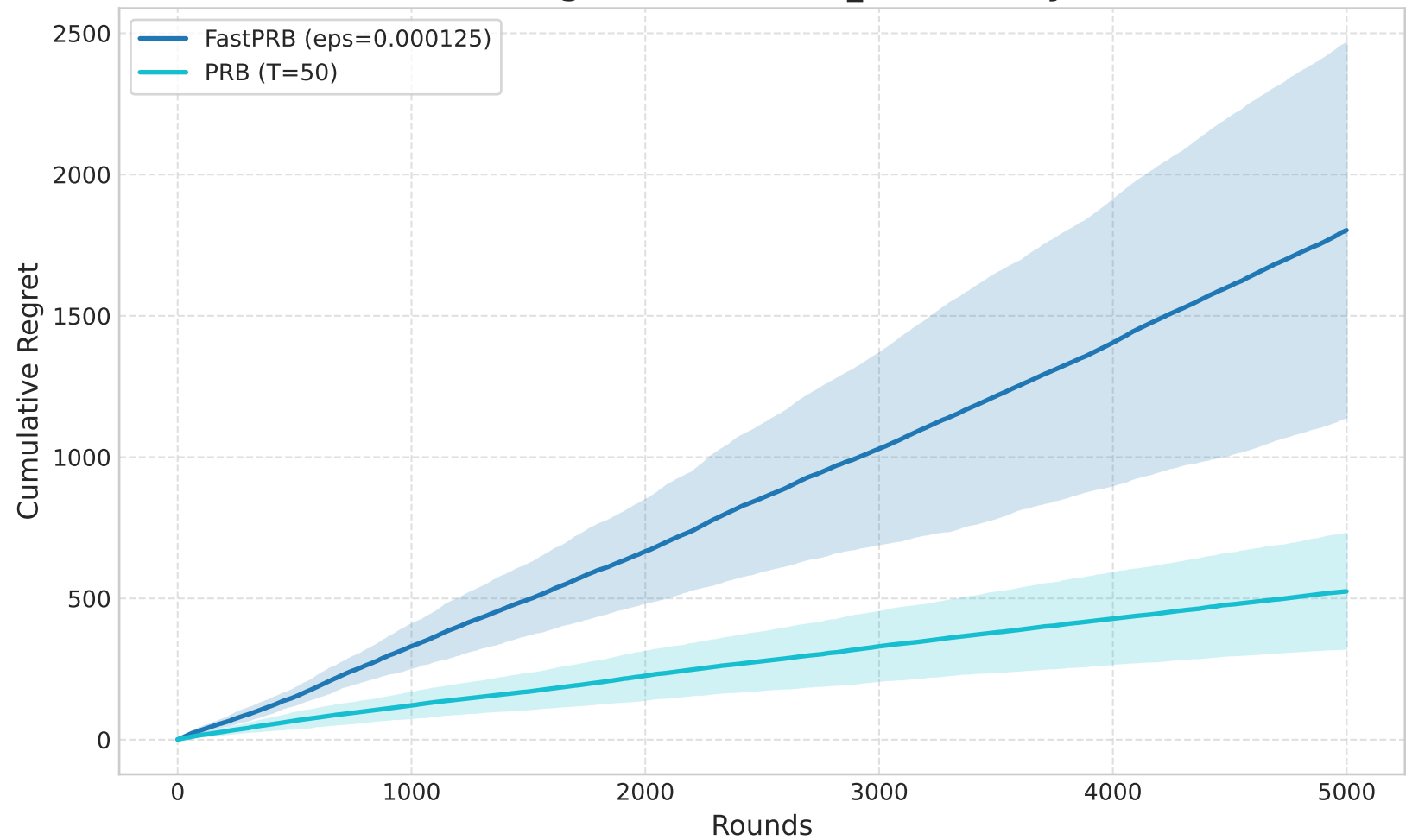
Cumulative Regret on Amazon_fashion (by Rounds)
