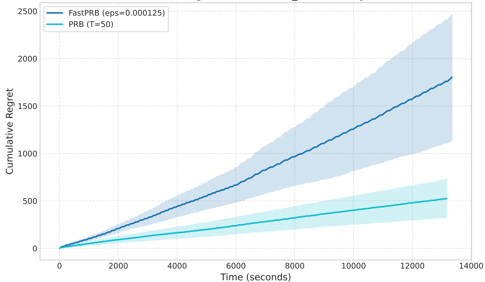
Cumulative Regret on Amazon_fashion (by Time)
