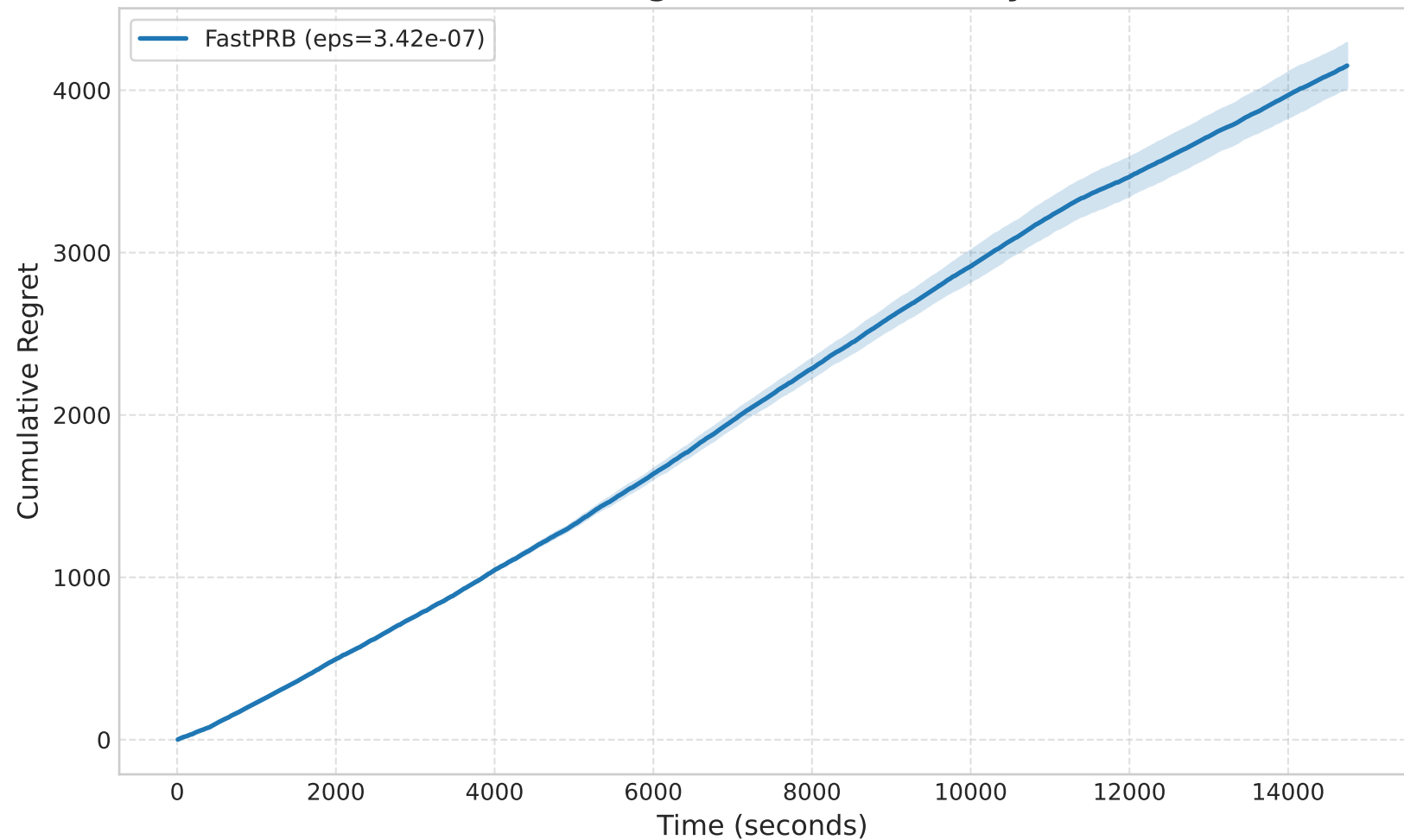
Cumulative Regret on Citation2 (by Time)
