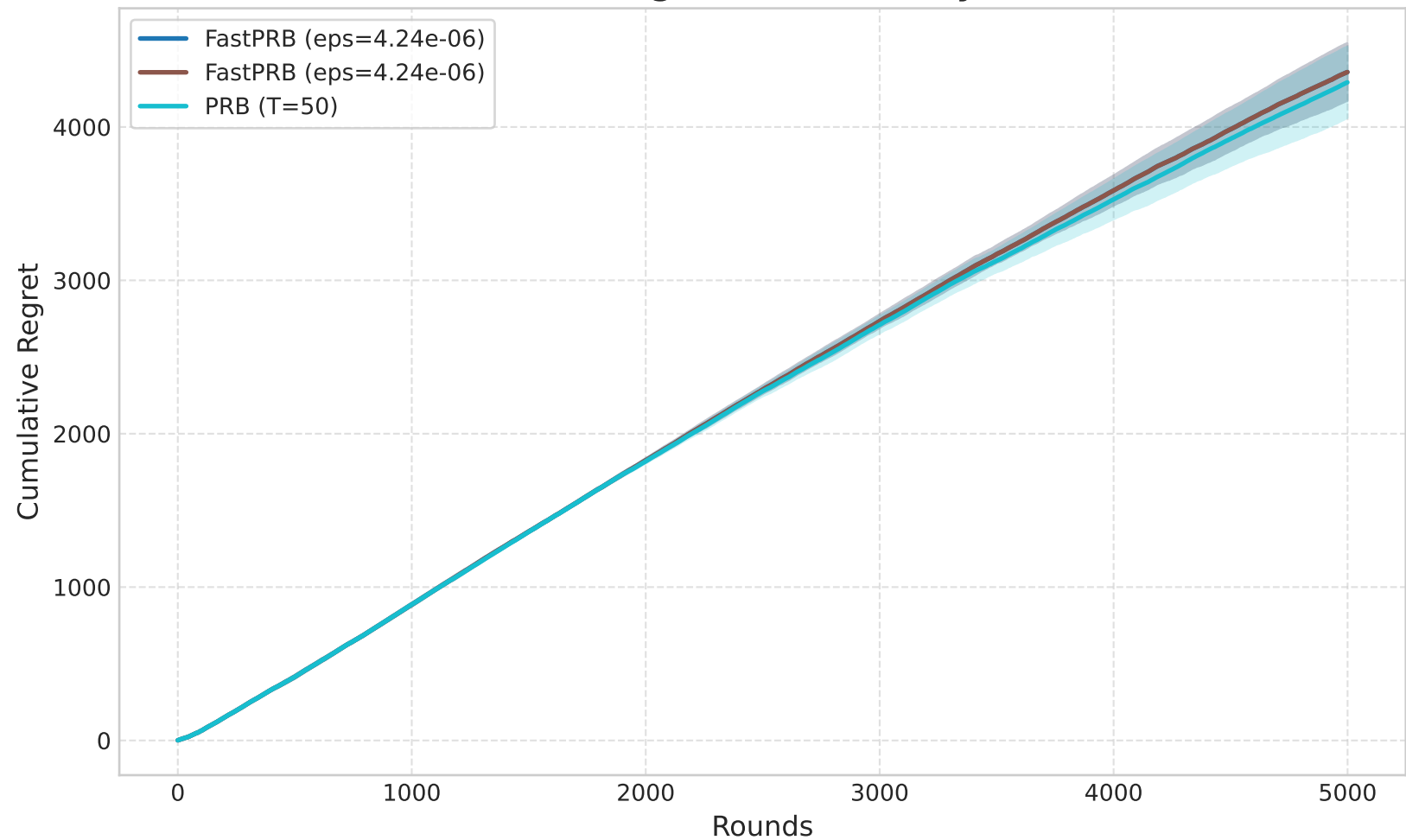
Cumulative Regret on Collab (by Rounds)
