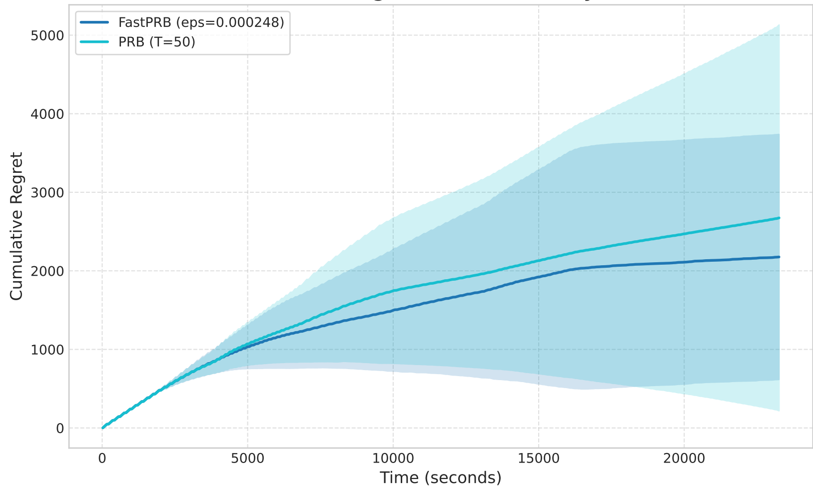
Cumulative Regret on Facebook (by Time)
