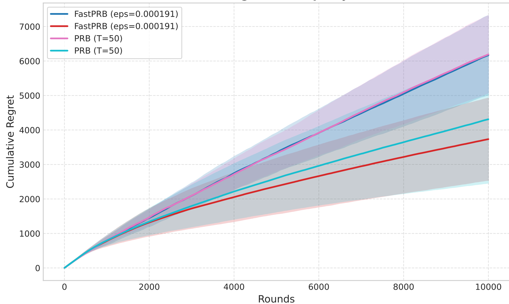
Cumulative Regret on Grqc (by Rounds)
