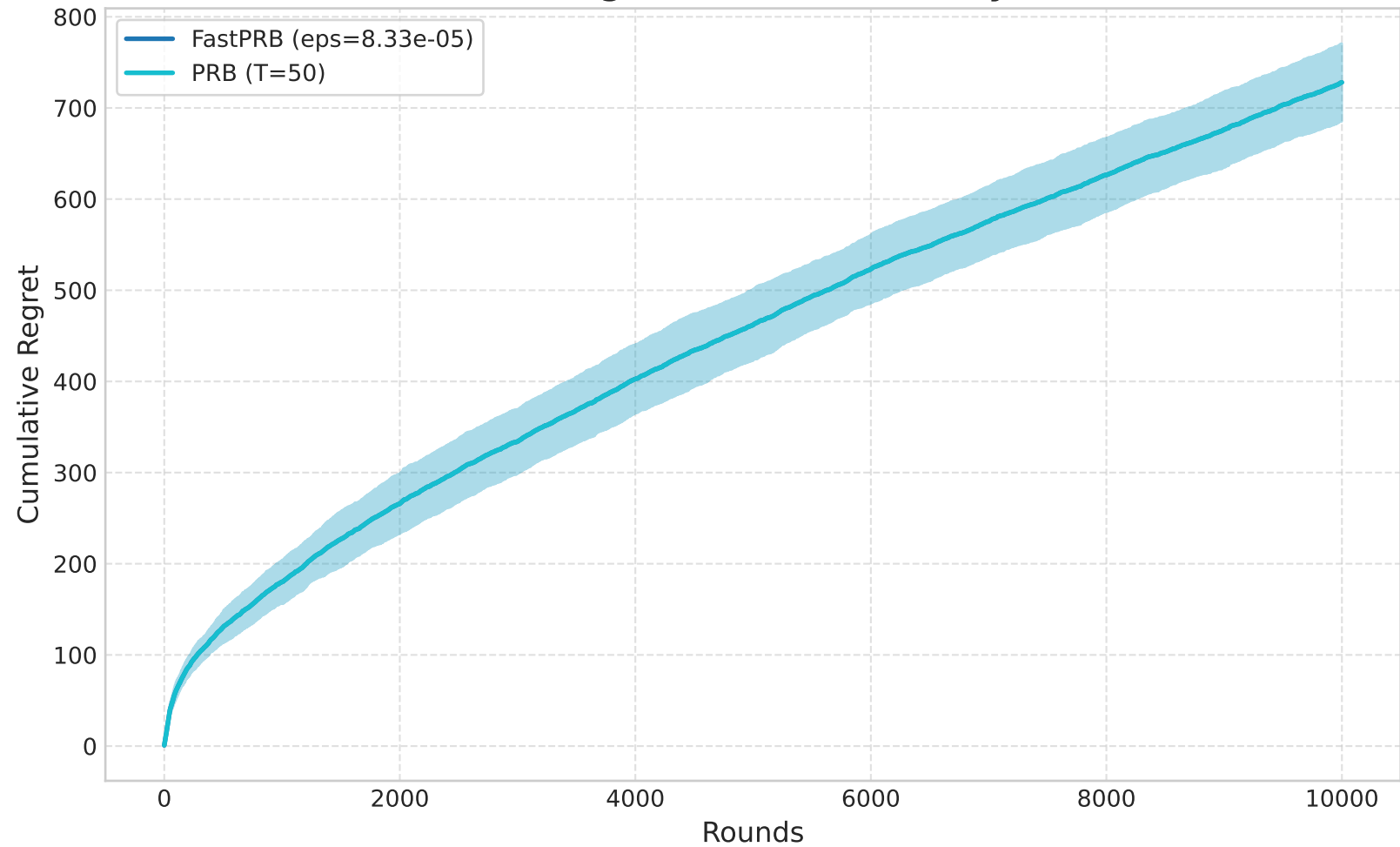
Cumulative Regret on MovieLens (by Rounds)
