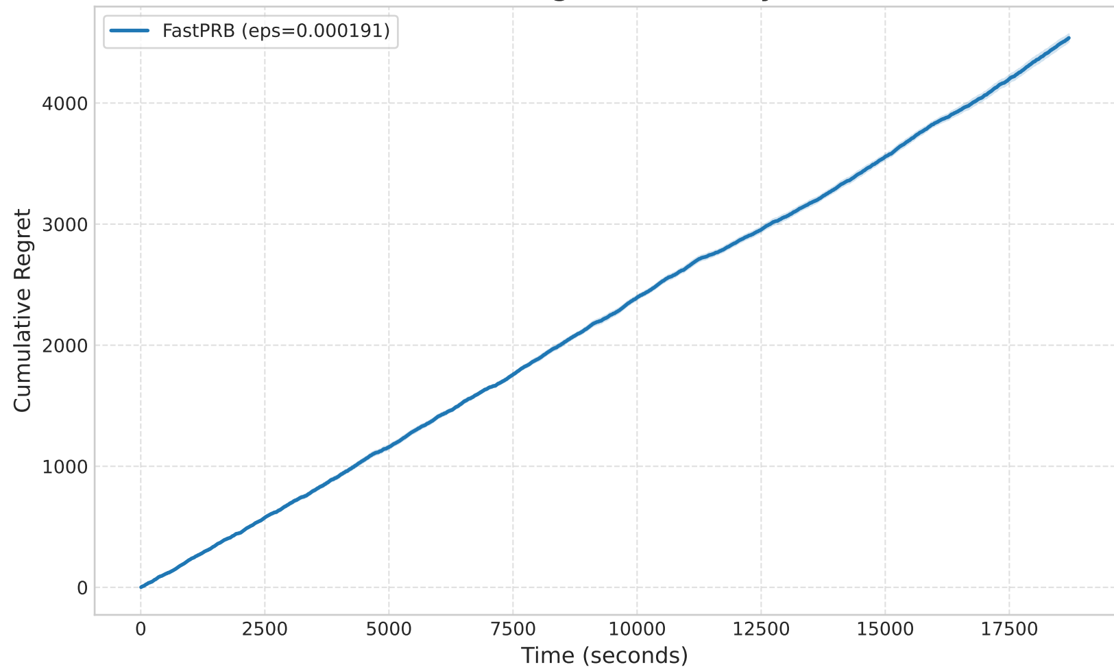
Cumulative Regret on PPA (by Time)
