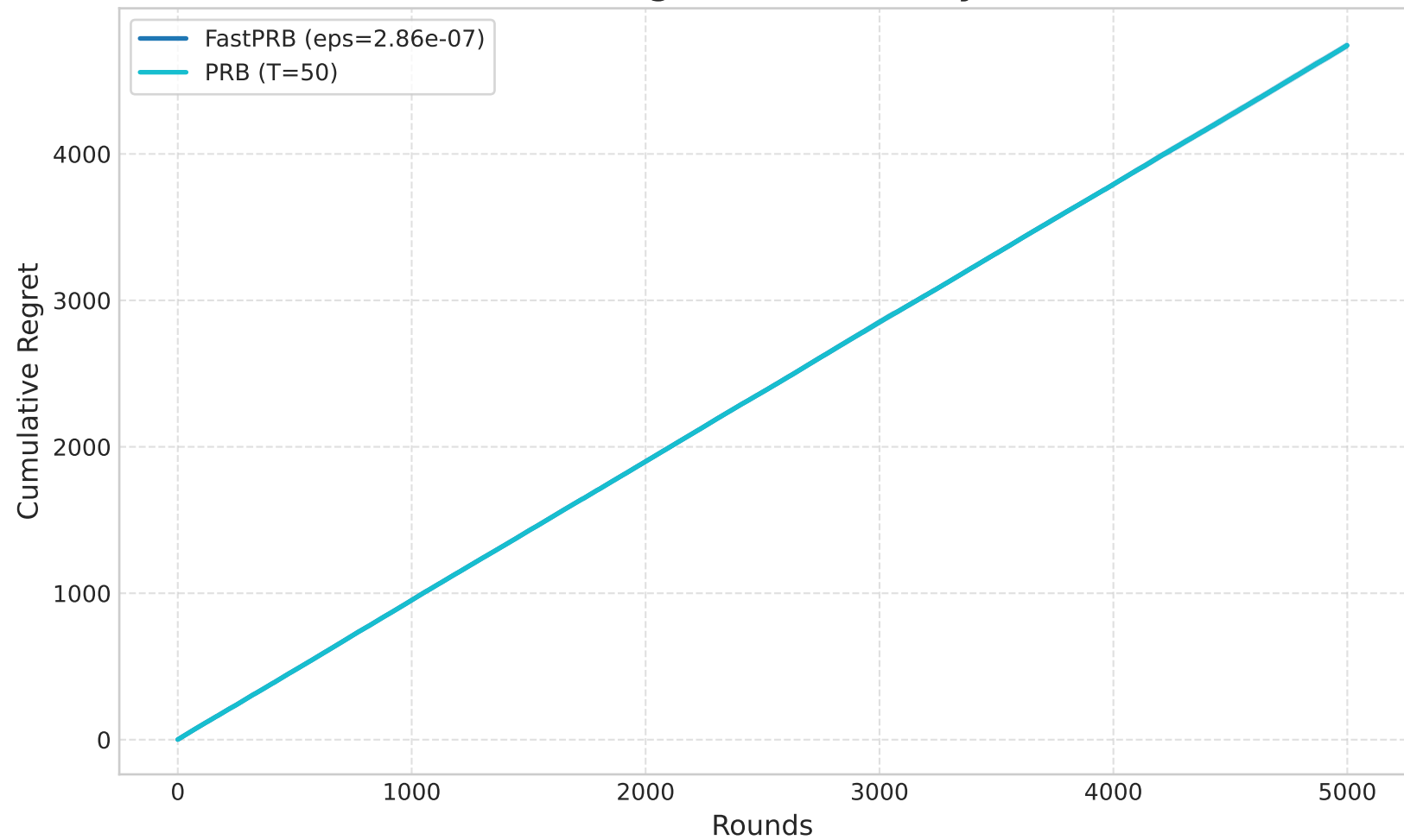
Cumulative Regret on Vessel (by Rounds)
