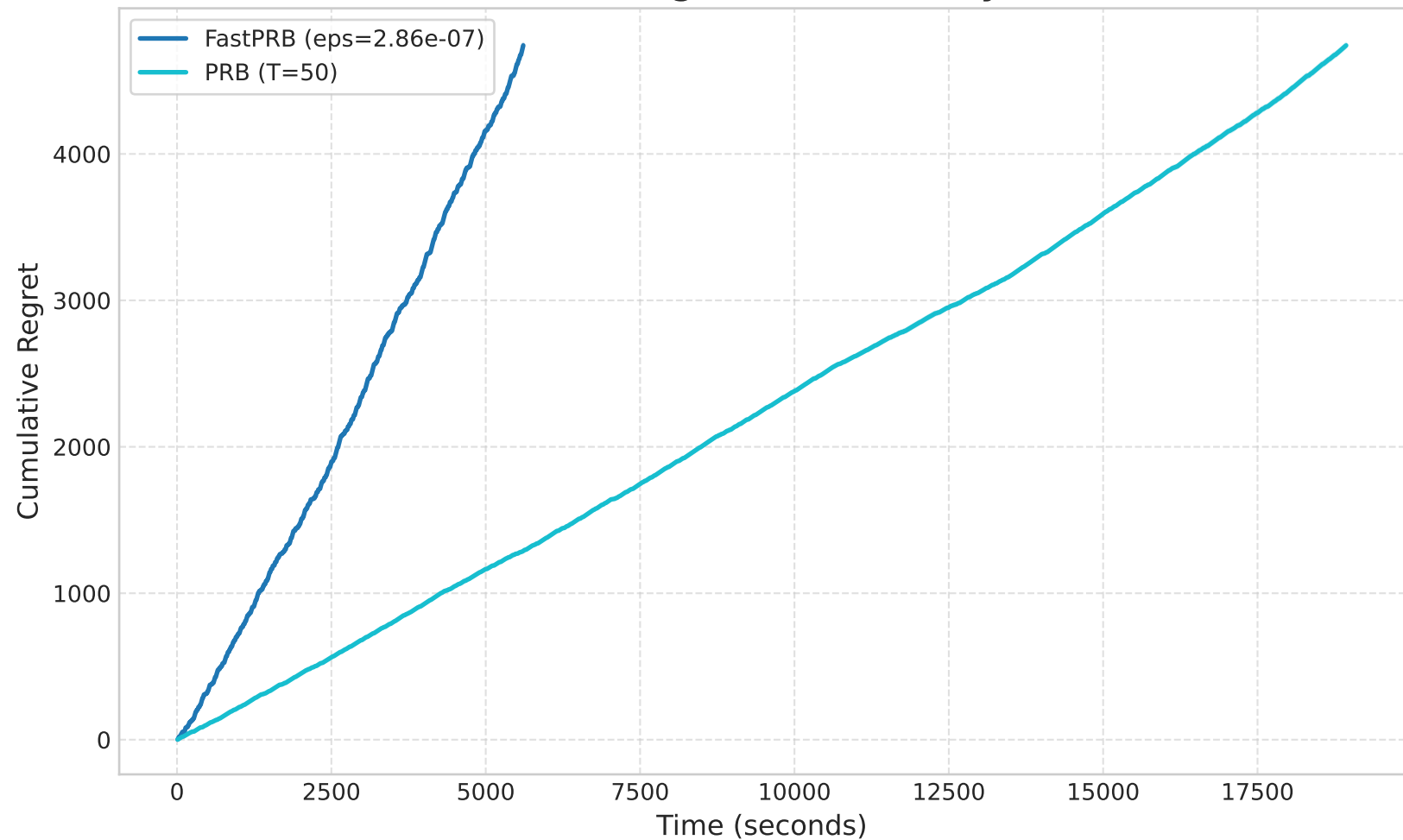
Cumulative Regret on Vessel (by Time)
