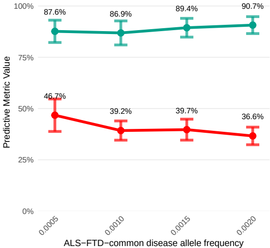
(E) Varying ALS-FTD-common disease allele frequency
