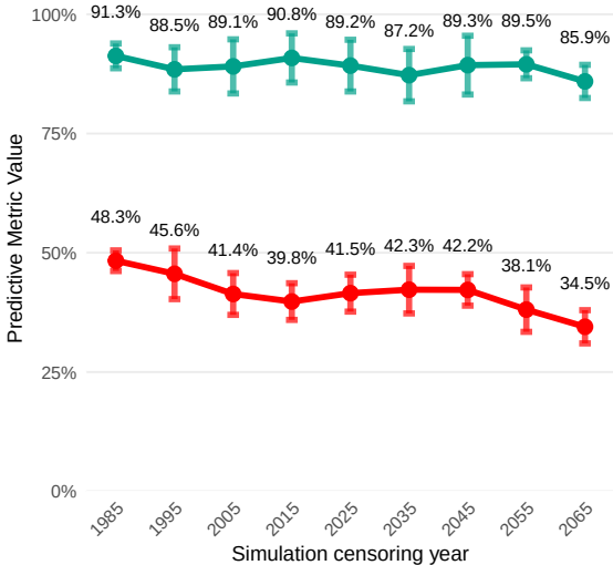
(L) Varying censoring years when running simulation
