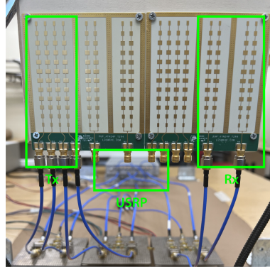
(b) Device layout at the JRC Station.
