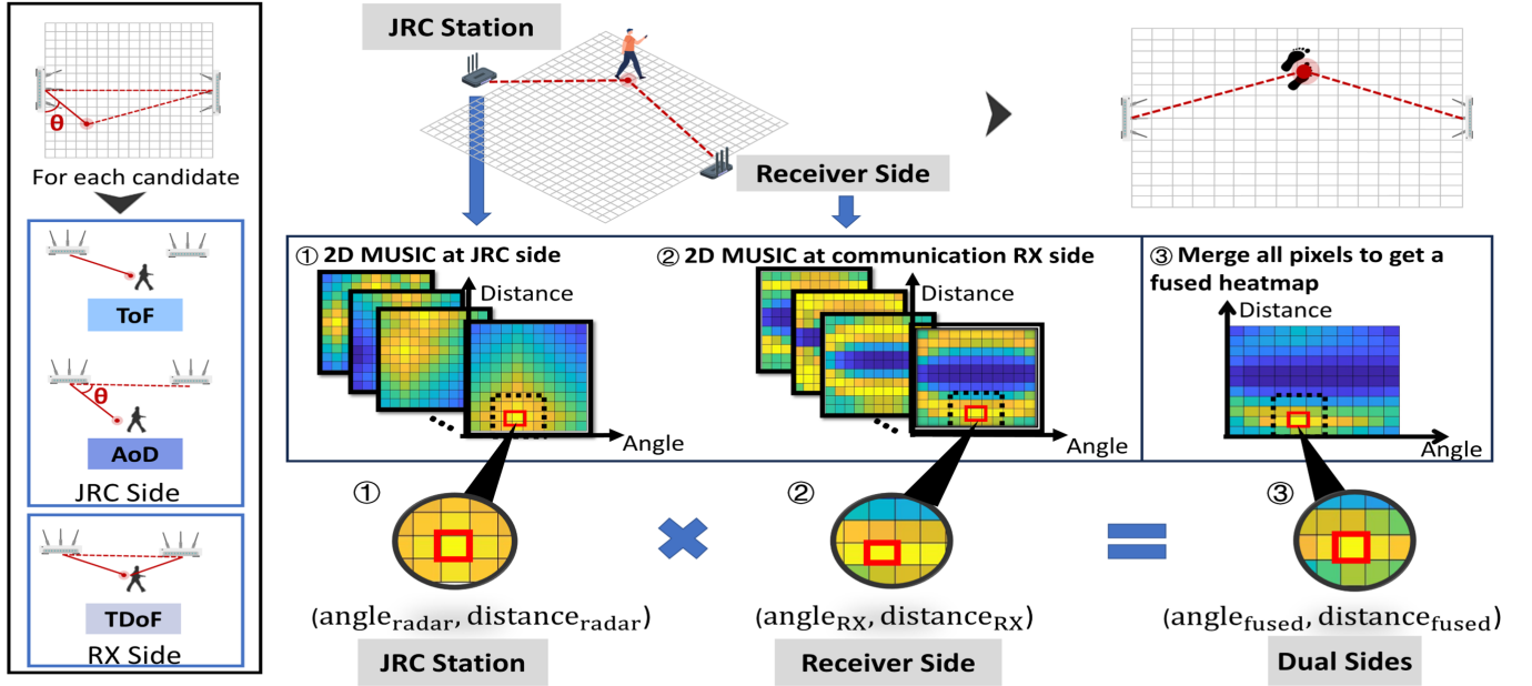
Fig. 4: Illustration of Heatmap Analysis and Fusion: The 2D-MUSIC method is applied independently on both the JRC and Receiver sides. Subsequently, the results are merged cell by cell to produce a comprehensive fused heatmap.
