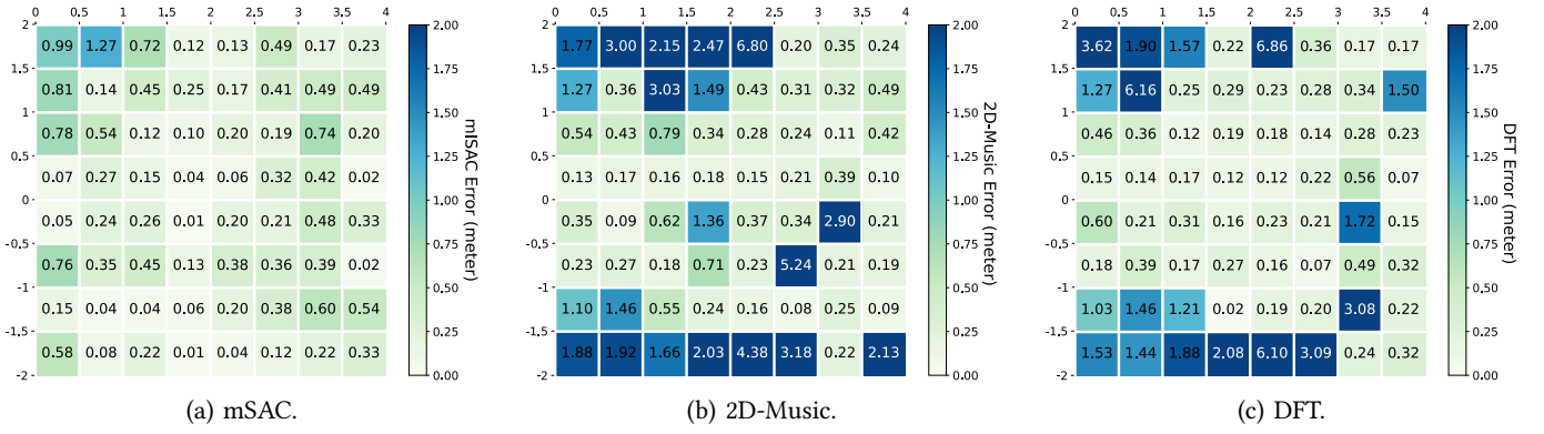
Fig. 7: Overall localization performance of mSAC , 2D-Music, and DFT.
