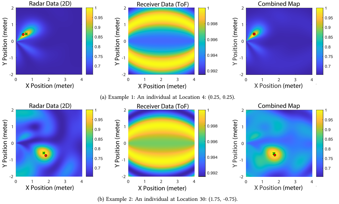
Fig. 6: Examples of mSAC localization results from the JRC station's radar side, Receiver side, and their combination.
