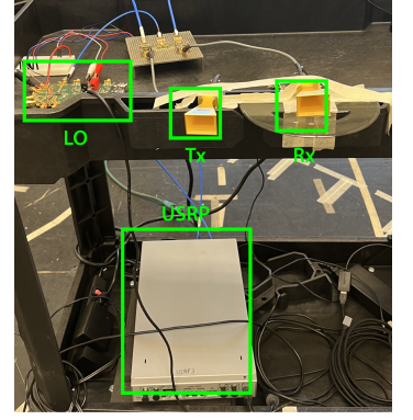
(c) Device layout at the Receiver Side.
