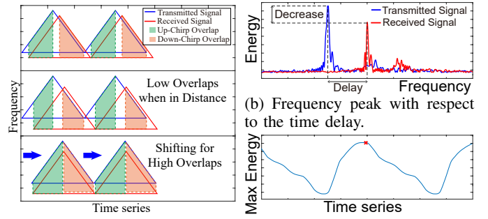
Fig. 6: Signal enhancement process.
