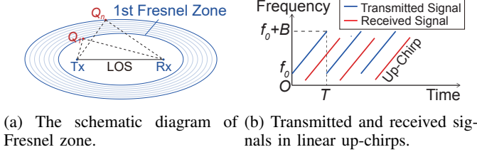
Fig. 2: Theoretical models in Wi-Fi and acoustic sensing.
