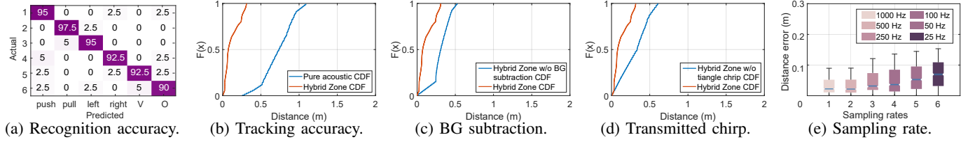
Fig. 13: Overall performance.
