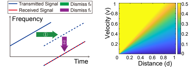
(a) Shifting for dismissing the dismissed signal ( f_d ) and velocity ( f_v ). (b) Proportion of velocity's influence on shift relative to distance.
