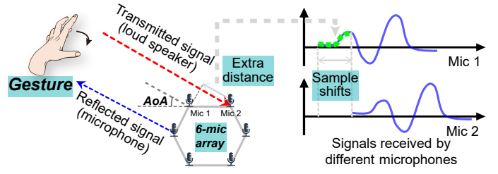
Fig. 7: The principle of AoA estimation.
