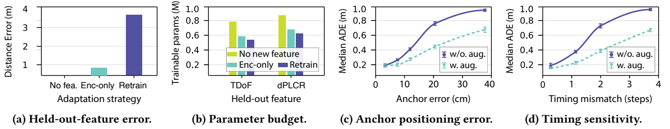
Figure 10: Feature-onboarding and mismatch-robustness studies in simulation.
