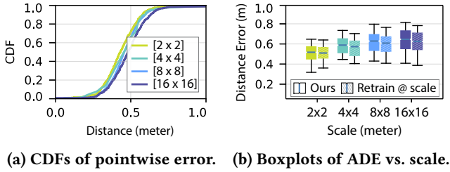
Figure 13: Real-world scaling experiments.
