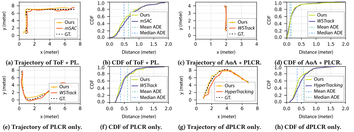
Figure 12: Real-world trajectory recoveries and pooled error CDFs for representative feature compositions.
