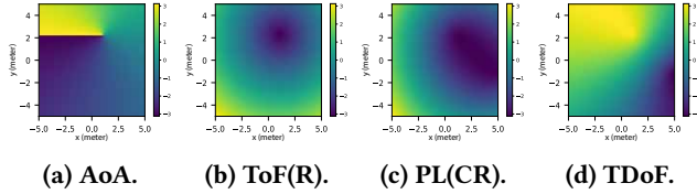
Figure 4: Representative spatial patterns of synthesized feature values across feature families in simulation.
