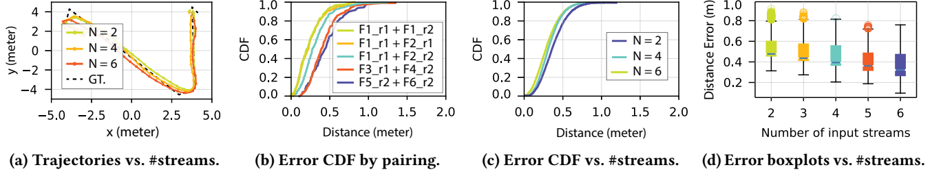
Figure 8: Simulation results under varying numbers of input streams and feature compositions.
