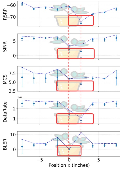
Figure 5: Representative per-metric LTE responses along the lateral scan axis. Each subplot shows one standardized link indicator.
