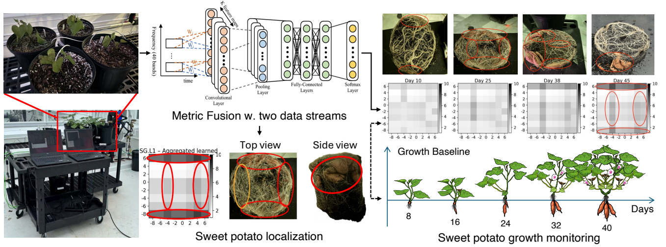
Figure 2: Overview of SWAMP. A repeatable SDR-based stepped-frequency sweep provides complex CFR measurements for longitudinal monitoring, while a private LTE link produces standardized link-quality indicators for localization and auxiliary condition sensing.
