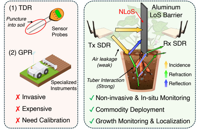
Figure 1: Motivation for SWAMP . Unlike TDR and GPR, SWAMP uses commodity aboveground radios to enable non-invasive subsurface monitoring and localization.
