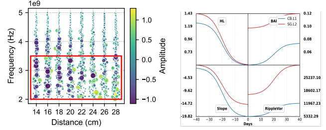
(a) Band selection from CFR sweeps. (b) Growth monitoring with CFR features.
