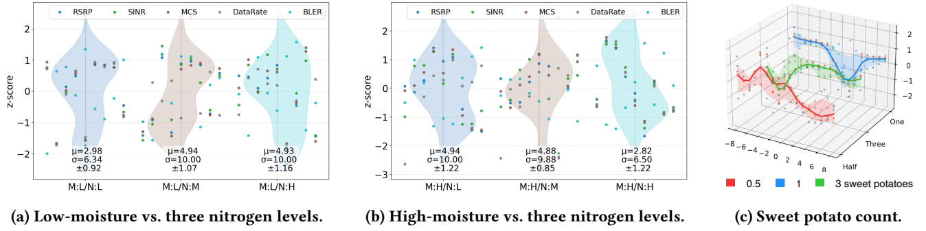
Figure 6: Auxiliary controlled studies using LTE-derived metrics.
