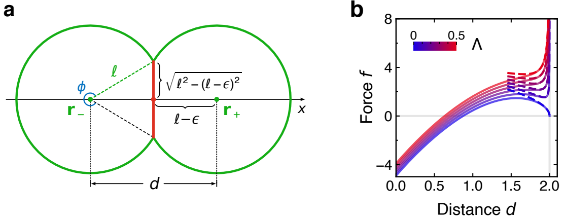
Figure 4.3: Cell doublet. a , Schematic of a cell doublet with centers positioned symmetrically at \mathbf{r}_{\pm} = \pm(\ell - \epsilon)\hat{x} . The arc radius of each cell is \ell , and the distance between the two cell centers is given by d = 2(\ell - \epsilon) , thus the contact length (red) is 2\sqrt{\ell^2 - (\ell - \epsilon)^2} . b , Force between a cell doublet as a function of their separation distance for \Lambda = 0, 0.1, 0.2, 0.3, 0.4 , and 0.5 (blue to red). Positive values f > 0 correspond to attractive forces. Solid lines show Eq. (4.6), and dashed lines are the asymptotic form for d \rightarrow 2\ell from Eq. (4.30). Default parameters: \ell = 1 , K_P = 1 , A_0 = \pi , and P_0 = 4.8 .
