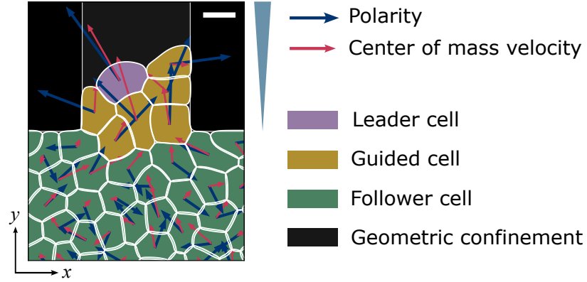
Figure 2.3: Schematic of the model. For each cell, the blue arrow represents its polarity \mathbf{P}_i , and the red arrow shows its center of mass velocity \mathbf{v}_i^{c.m.} ; chemoattractant concentration increases in the +y direction. Scale bar, 15 \mu\text{m} .
