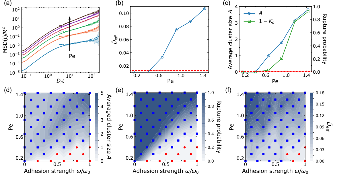
Figure 2.9: Unjamming and rupture. (a) Mean squared displacement MSD(t) for different cell motility quantified by a dimensionless Péclet number Pe := p_0/(RD_r) . The different Pe shown in this panel are 0.14, 0.40, 0.66, 0.91, 1.17, and 1.43 (default); we have rescaled MSD and t to make them dimensionless; for each Péclet number, the dashed lines are results from three independent simulations, and the solid line is their average, and the dash-dotted lines are linear fit at late times where the effective diffusivity \bar{D}_{eff} is extracted. (b) The effective diffusivity \bar{D}_{eff} as an order parameter for solid-liquid transition. (c) Corresponding rupture transition of average cluster size (blue) and rupture probability (green). Panels (d) and (e) are phase diagrams for rupture transition. Red points indicate values equal to 0 and blue squares represent values greater than 0. (f) Phase diagram for jamming transition. Red points indicate values below the threshold value 0.012 and blue squares represent values above the threshold value. 300 independent simulations for each point in panels (c)–(f).
