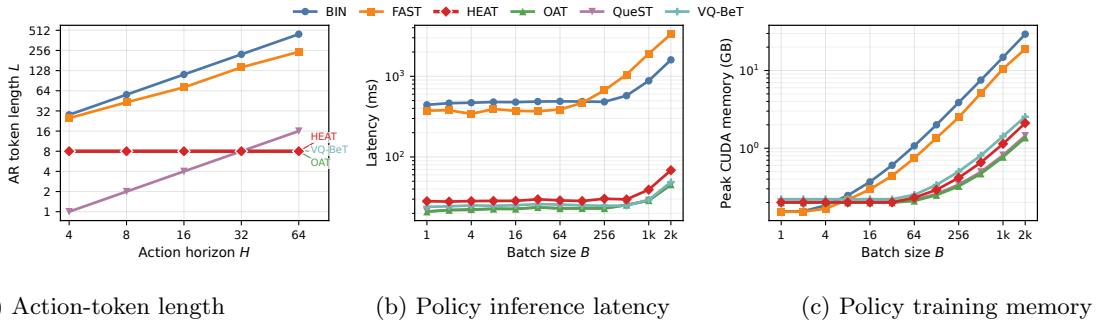
Figure 8: Complexity scaling for HEAT and its matched action-representation baselines; Continuous-HEAT is not included. (a) Autoregressive action-token length as the horizon grows. Binning scales as HD_a , FAST follows its measured BPE length, HEAT, OAT, and VQ-BeT use a fixed eight-token interface, and QueST grows as H/4 . (b) Policy inference latency at H = 32 . Long coordinate-level and BPE sequences dominate generation cost, while compact event or latent interfaces remain much flatter. (c) Peak CUDA memory during policy training at H = 32 . The memory of binning and FAST grows rapidly with batch size because their action-token sequences are long.
