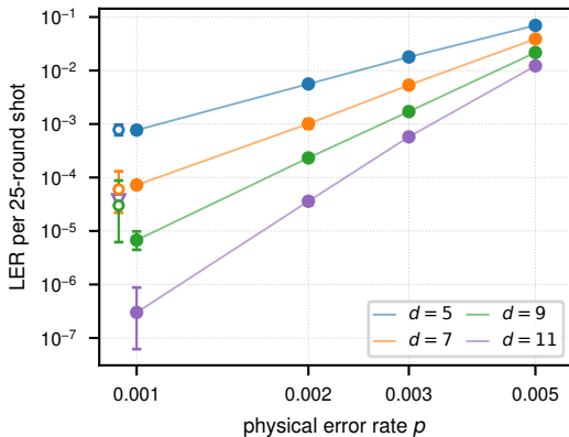
C BB codes, BP-OSD, phenomenological
