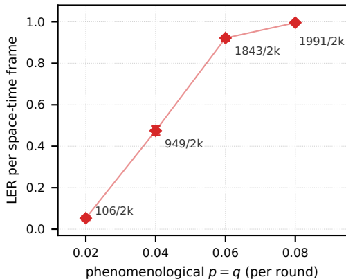
C [[72, 12, 6]], BP-OSD, phenomenological, T = 6
