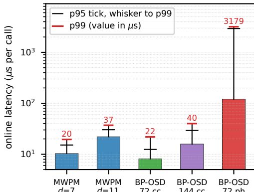
D online single-shot latency
