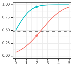
psymetadata psychology
