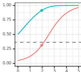
OpenSciCollab psychology
