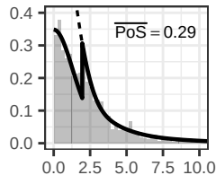
clinicaltrials.gov Phase 4
