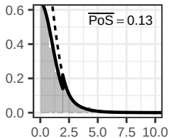
CDSR Stroke
