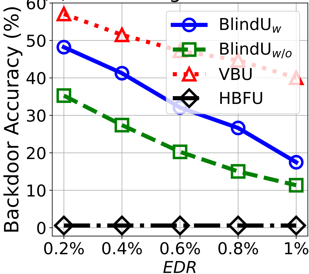
(k) Unlearning Effectiveness
