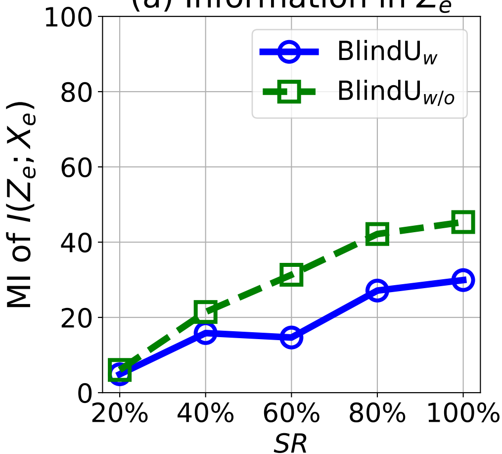
(a) Information in Z_e
