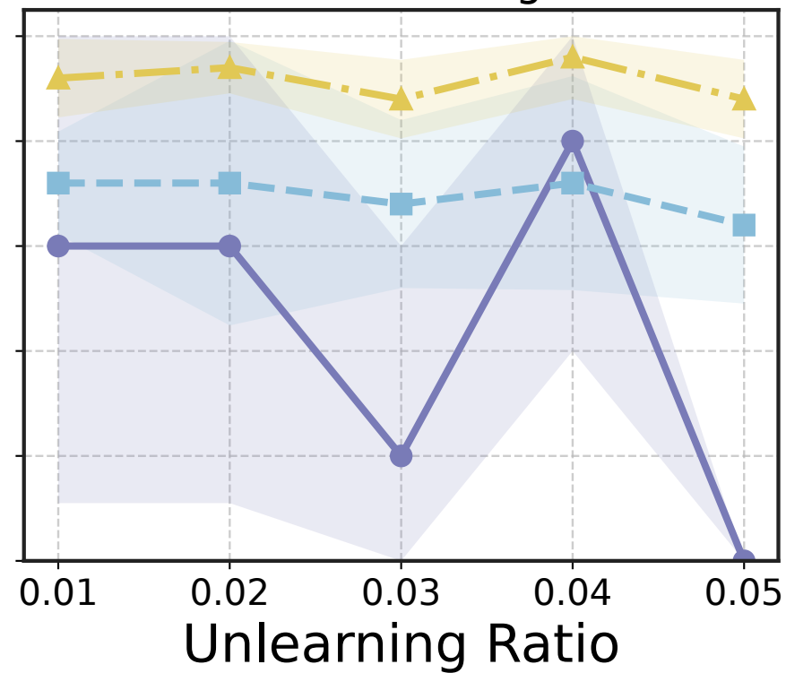
FL Retraining
