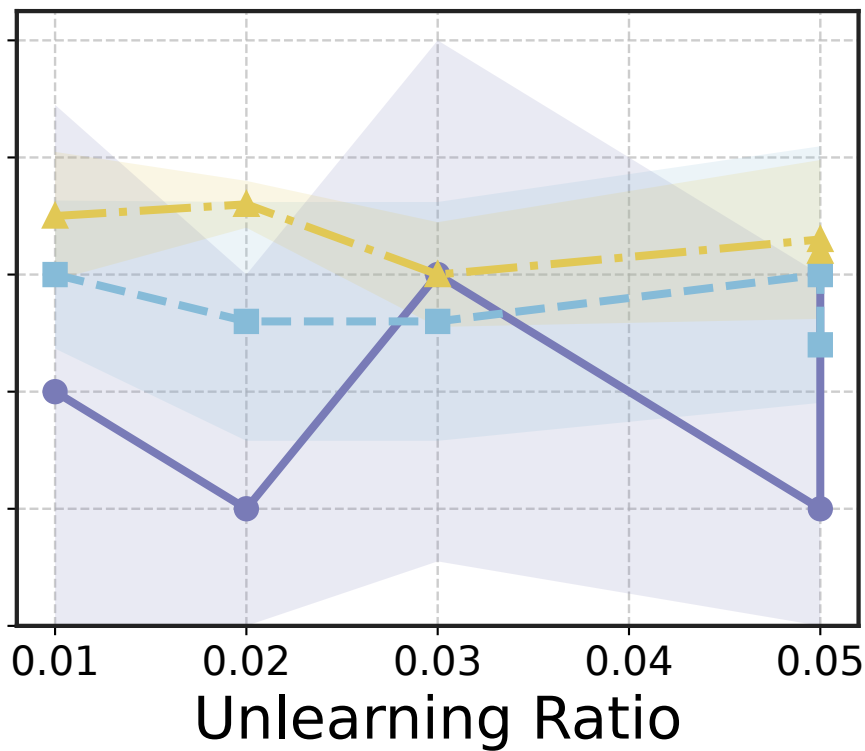
Hessian-FU
