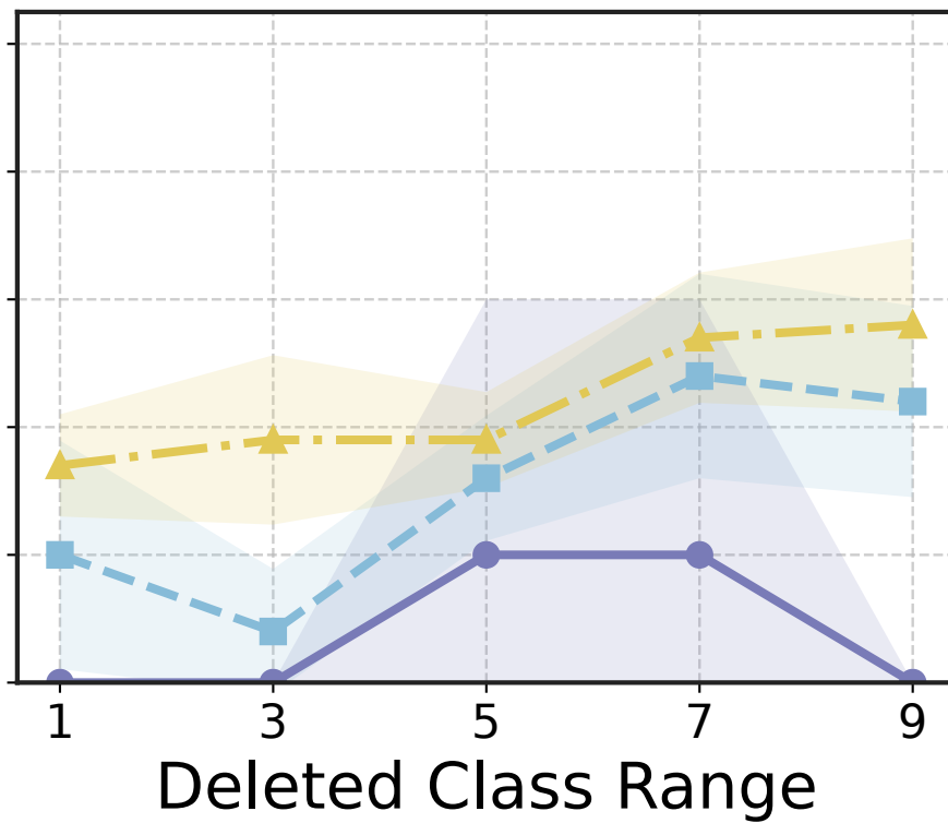
Hessian-FU
