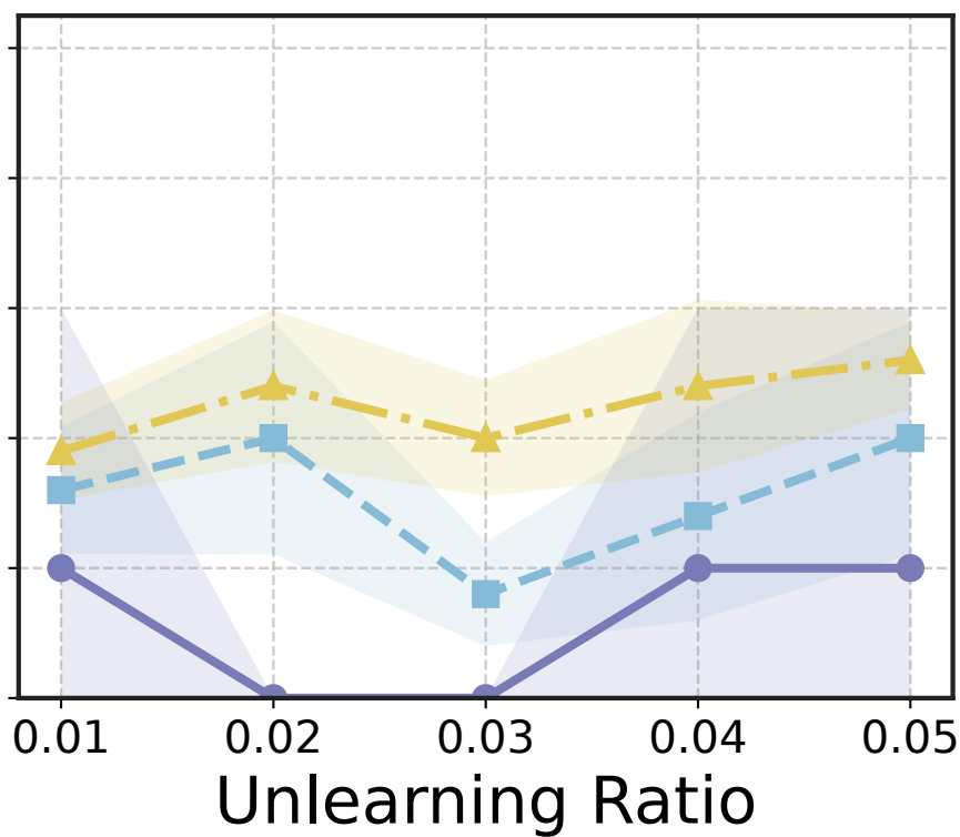
Hessian-FU
