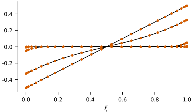
\hat{s}_G(\xi, \tau) : series (line) vs FDM (dots)
