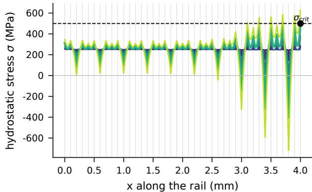
(a) stress profiles (thin grey lines: feeds)
