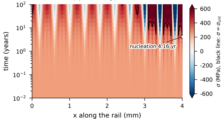
(b) stress map, all times
