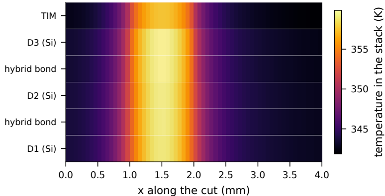
(a) vertical cut at y = 1.53 mm through the D3 hot spot (layer heights not to scale)
