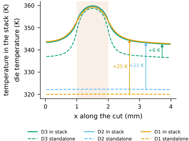
(b) along the cut: in the stack (solid) vs standalone (dashed)
