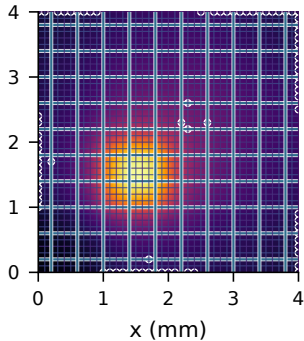
D2 (4 W) earliest 5.20 yr
