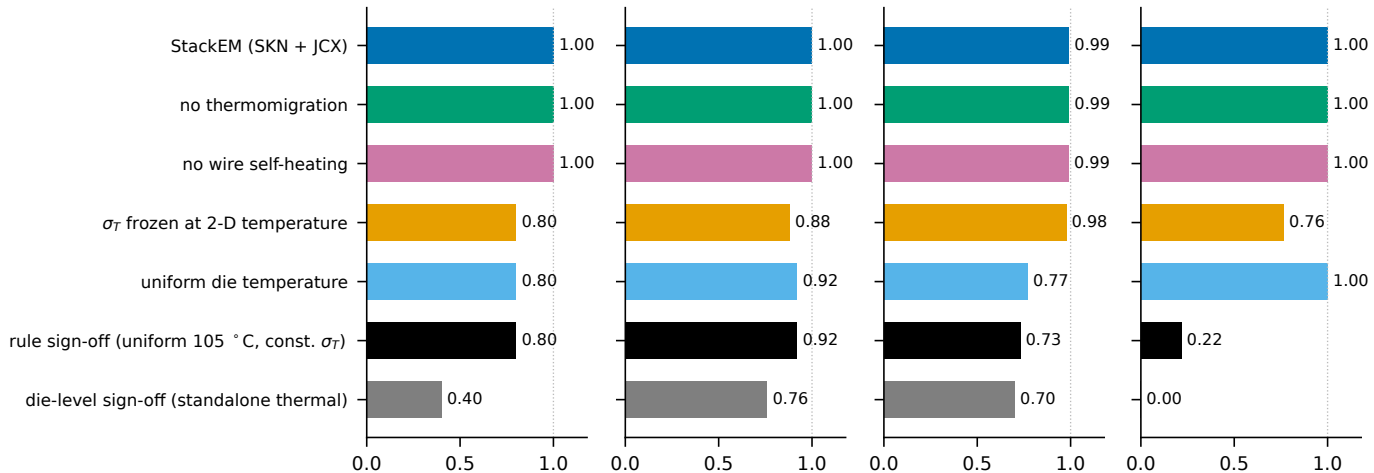
mortal set (10 yr) Jaccard
