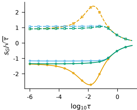
s_G/\sqrt{\tau} at both ends
