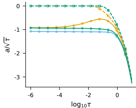
a/\sqrt{\tau} at both ends
