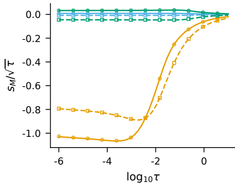
s_M/\sqrt{\tau} at both ends
