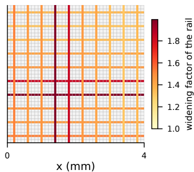
D2: 20 / 82 rails violate 10 yr
