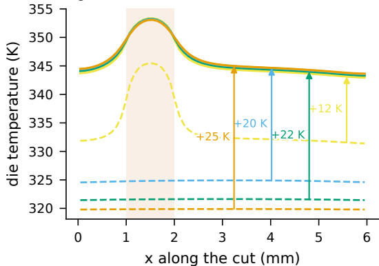
(b) along the cut: in the stack (solid) vs standalone (dashed)
