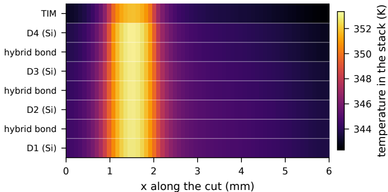
(a) vertical cut at y = 4.45 mm through the D4 hot spot (layer heights not to scale)
