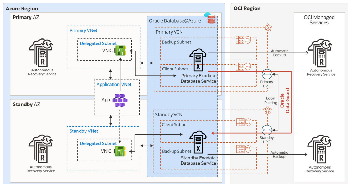
Figure 35-4 MAA Gold DR Architecture in the Same Azure Region
