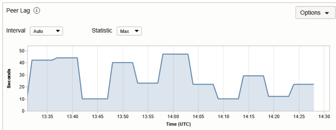
Figure 33-2 Peer Lag for Cross-Region Standby
