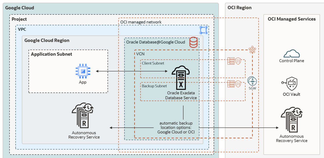
Figure 35-6 MAA Silver Architecture for Oracle Database@Google
