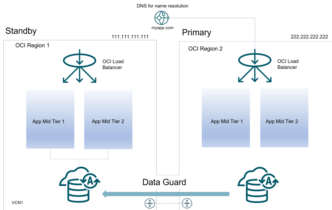
Figure 40-2 Sites after switchover
