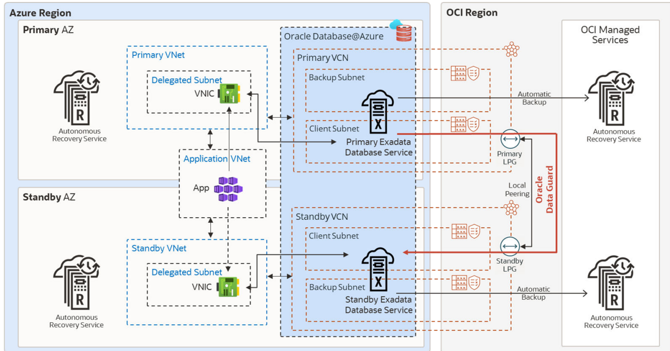
Figure 35-2 MAA Gold DR Architecture in the Same Azure Region
