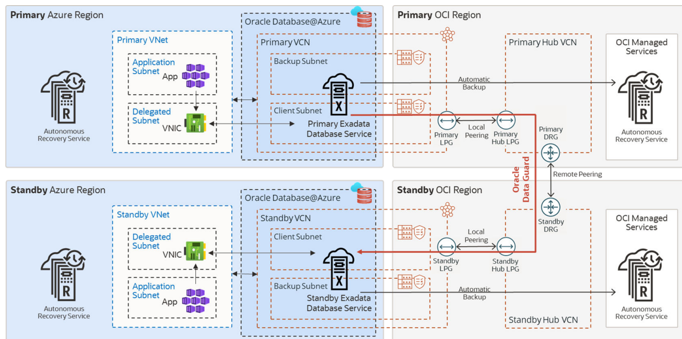
Figure 35-5 MAA Gold DR Architecture Across Two Azure Regions
