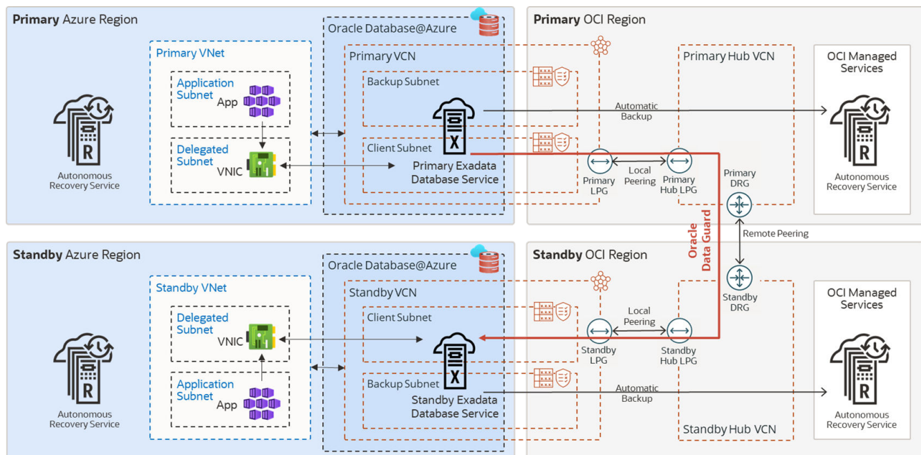
Figure 35-3 MAA Gold DR Architecture Across Two Azure Regions
