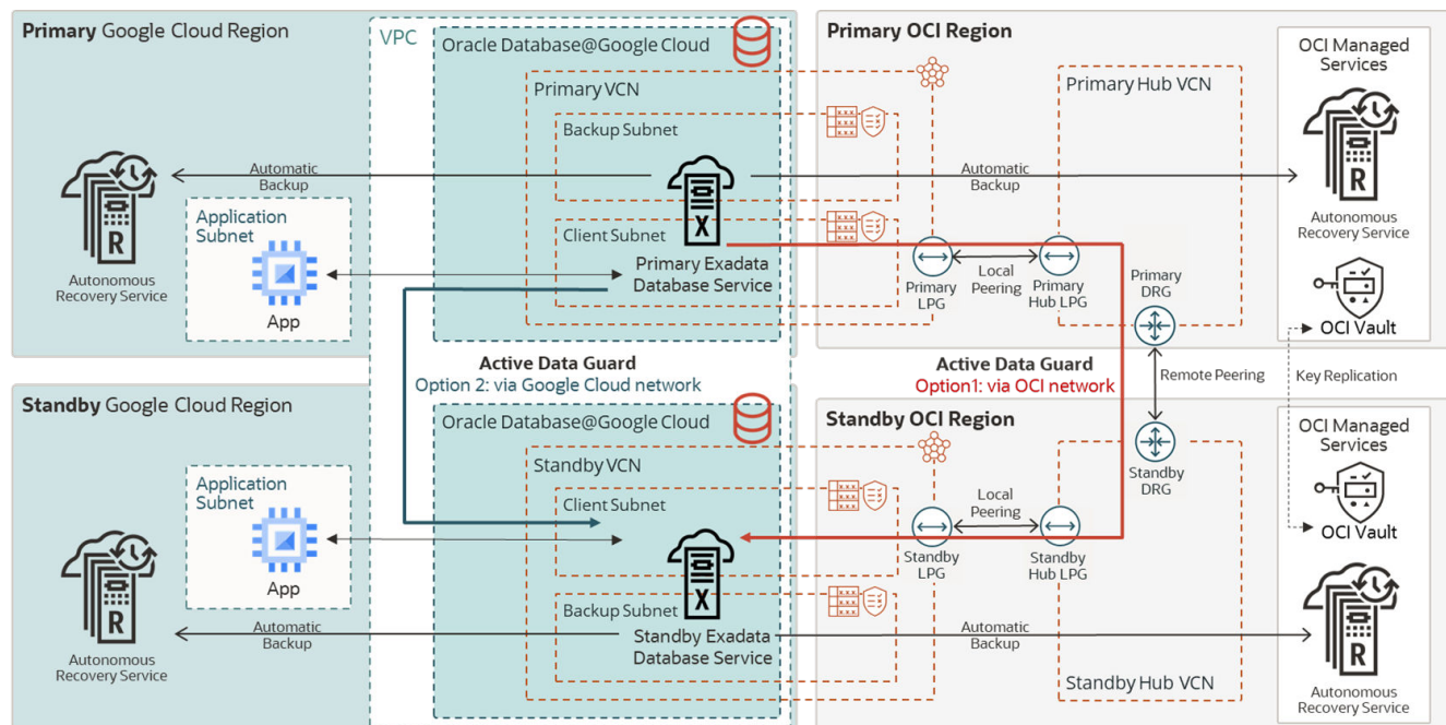
Figure 35-7 MAA Gold Architecture for Oracle Database@Google
