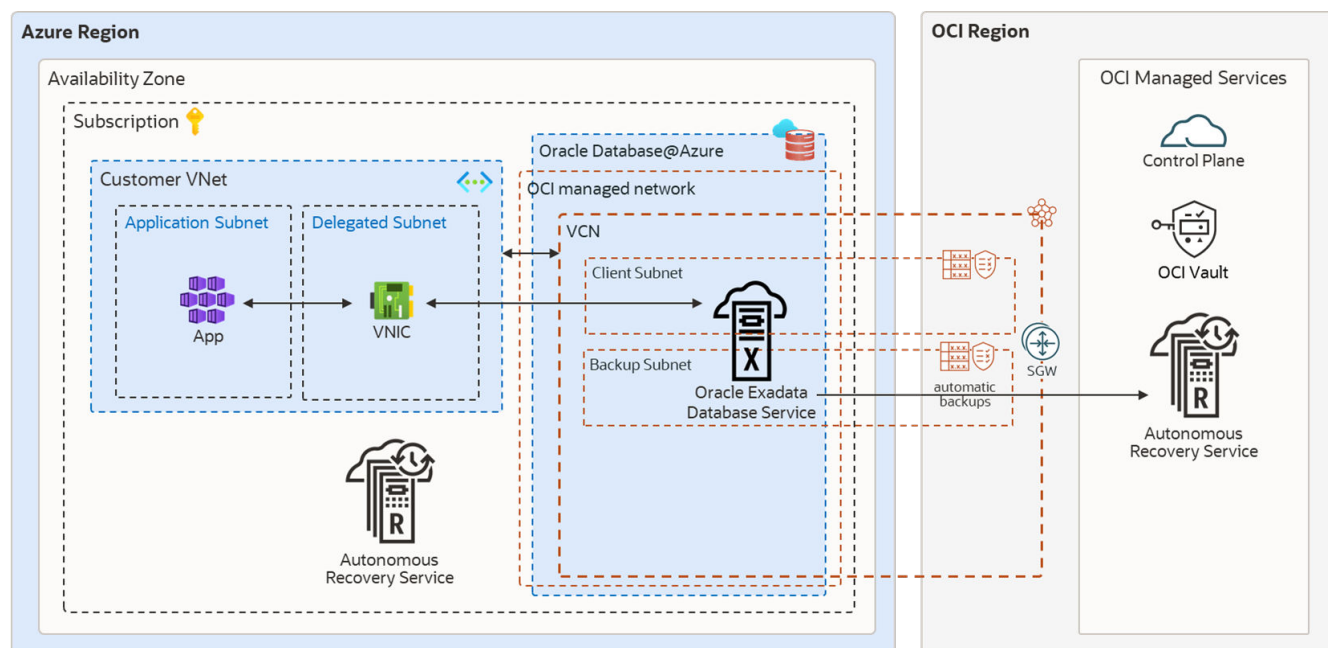
Figure 35-1 MAA Silver Architecture for Oracle Database@Azure
