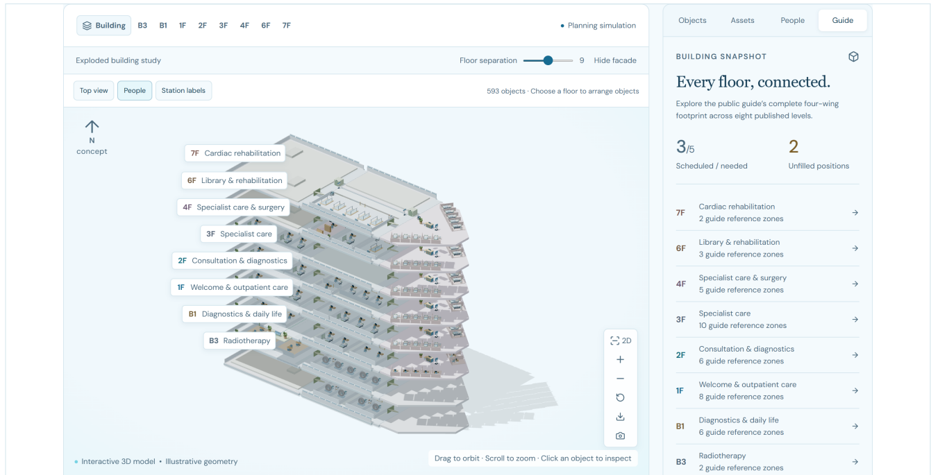
FIG. 2 Explore the demonstration building. An exploded 3D view connects eight modeled levels with service locations; each floor can be opened for detailed inspection.
