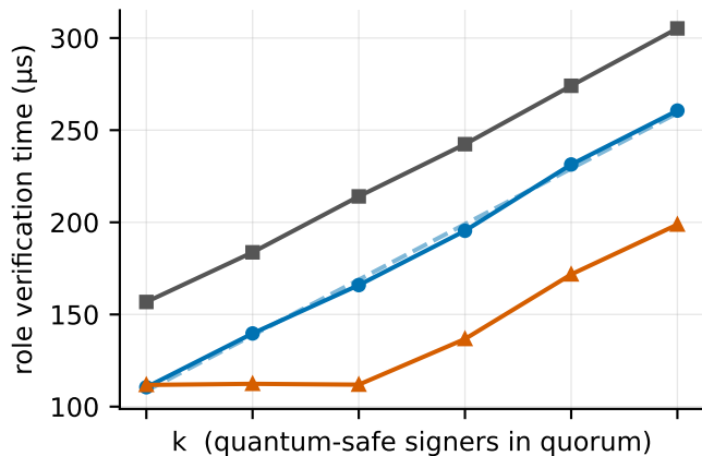
FN-DSA-512 — avx2
