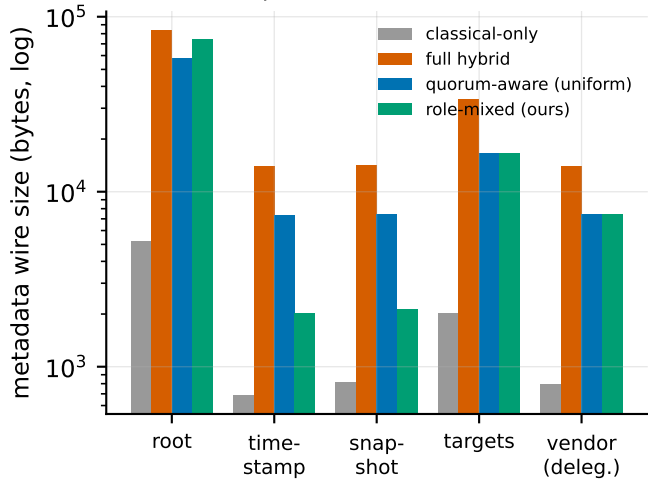
(a) per-role metadata size
