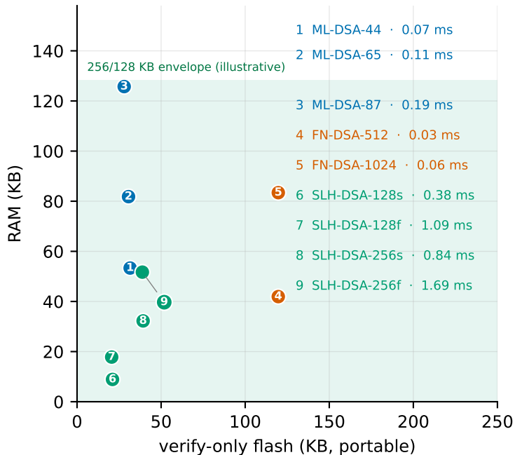
(b) MCU flash/RAM envelopes (portable)
