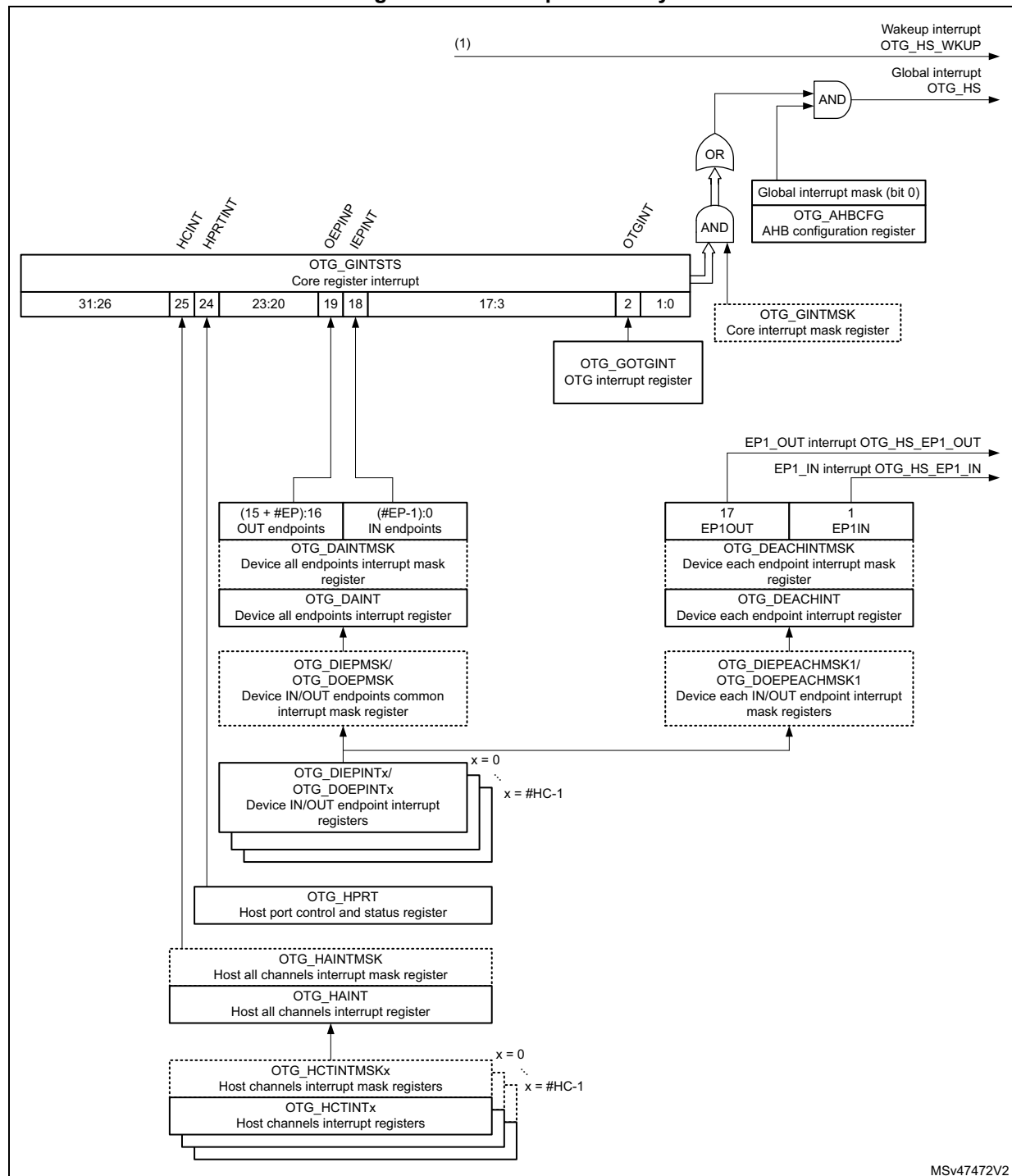
Figure 414. Interrupt hierarchy
