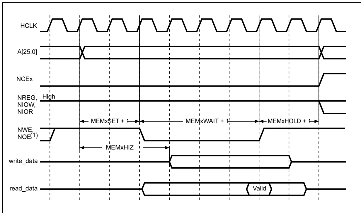
Figure 454. NAND/PC Card controller timing for common memory access
