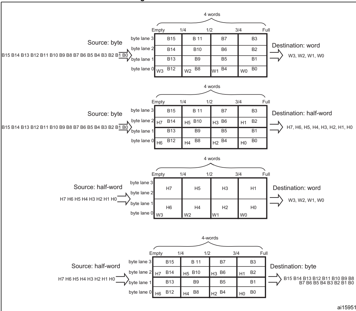
Figure 39. FIFO structure
