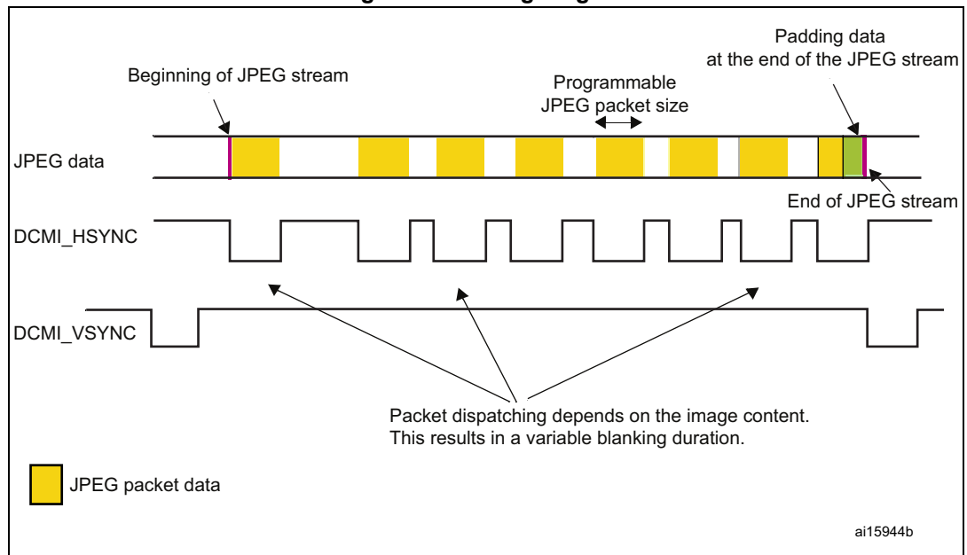
Figure 75. Timing diagram
