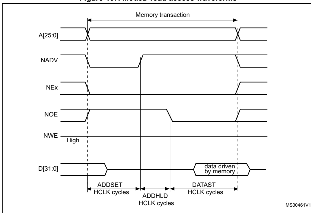
Figure 467. ModeD read access waveforms
