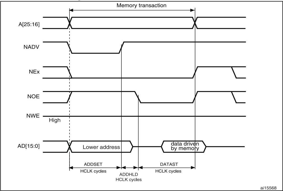
Figure 469. Muxed read access waveforms
